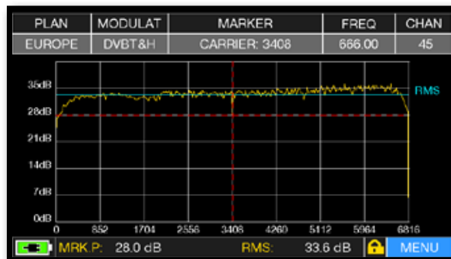
MER vs CARRIER : visualization mode "VIS. TYPE: NORMAL" & "PICTURE: CONTOURS".
