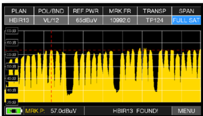
SAT spectrum SPAN "Full SAT" (from 930 to 2250 MHz).
