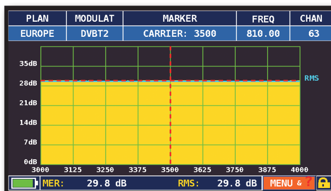
MER vs CARRIER: Visualization mode "VIS. TYPE: NORMAL", "PICTURE: FULL" and "START/STOP CARR from 3000 to 4000".
