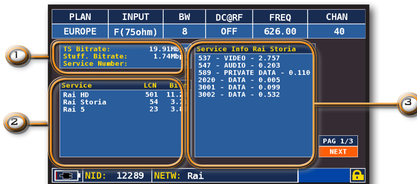
Pages 1/3: Transport stream bitrate monitoring
