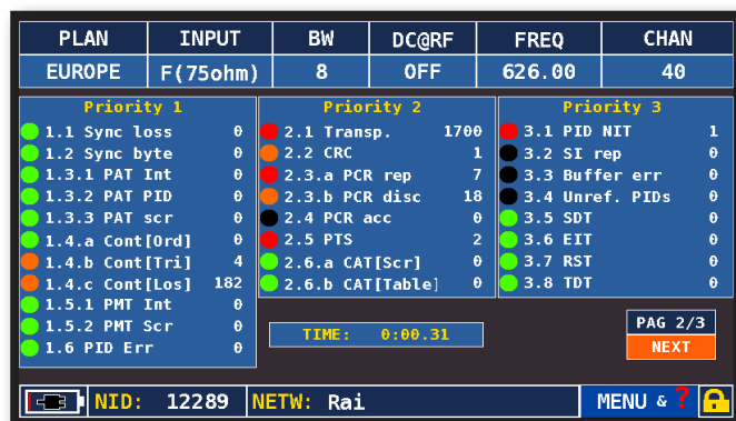
Pages 2/3: ETR101290 analysis
