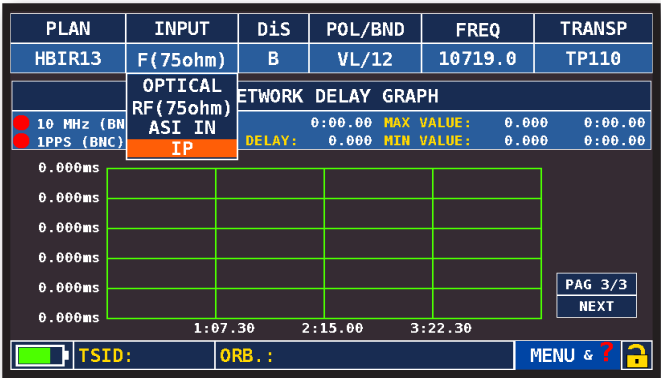
Touch "INPUT" and select "IP" and wait for the IP board to start up
