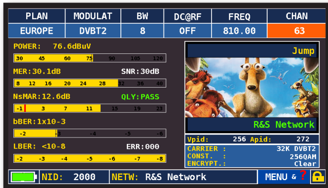
Main measurements and picture
