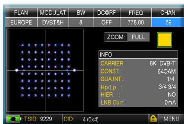
Fig. 4: DVB-T-64Q CONSTELLATION: The table to the right shows all the received modulation parameters
