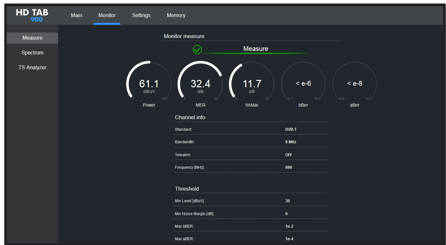
Example of MEASUREMENTS of a TV CHANNEL (DVB-T Standard) And related screen of IMPULSE RESPONSE (ECHOES)
