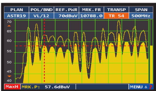
Fast spectrum with peak memory "Max HOLD"
