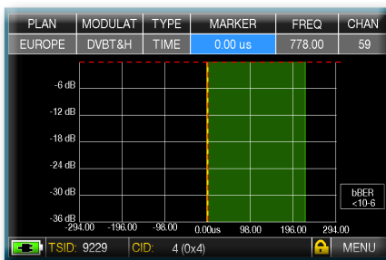
Fig. 1: OPTIMUM RECEPTION:* no ECHO present either outside or inside the guard interval mask (green area).
