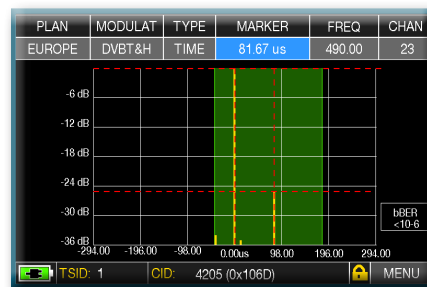
Fig. 2: GOOD RECEPTION:* 2 ECHOES present, but within the guard interval mask (green area) coming from a distance of: 1st echo: 24,50 Km, the same as a 81,67 \mu\text{s} delay.
