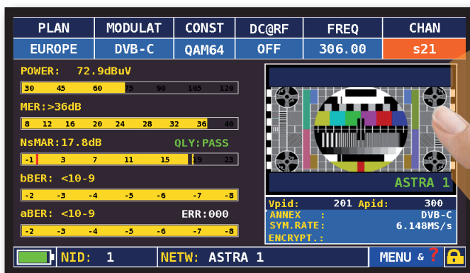
Main measurements & live picture
