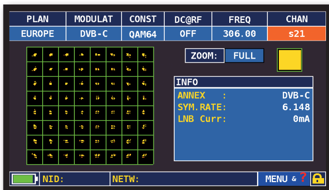
64 QAM constellation
