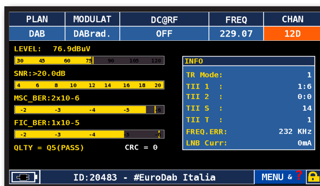
Main DAB measures
