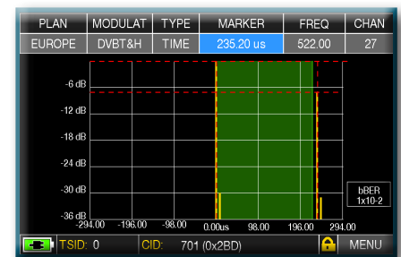
Fig. 3: MARGINAL RECEPTION (or IMPOSSIBLE):* 2 ECHOES present outside the guard interval mask (green area), coming from a distance of: 1st echo: 70,56 Km, the same as a 235,20 \mu\text{s} delay.
