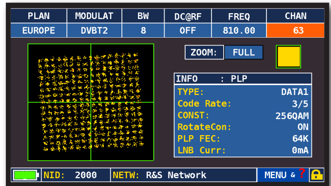
DVB-T2 constellation
