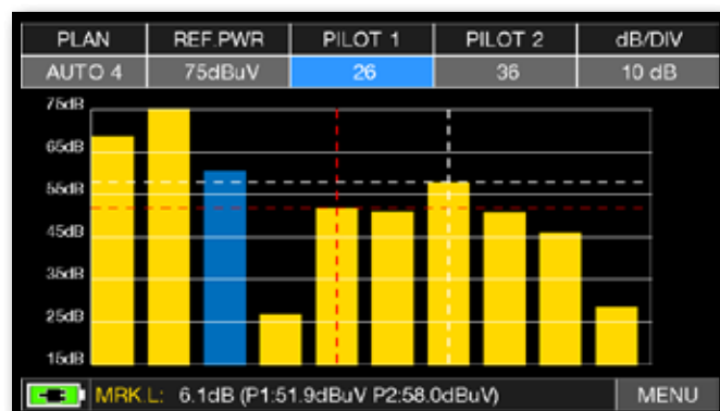
BARSCAN (TILT GRAPHIC).
