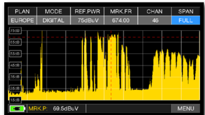
TV SPAN FULL spectrum with mixed channels SAT signals (from 5 to 1.250 MHz).
